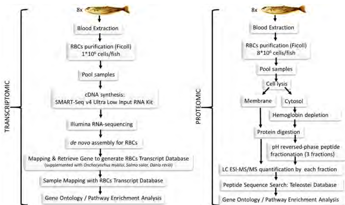
Figure 1. Schema representing the different steps in the experiment described here, from sample collection to data analysis.
